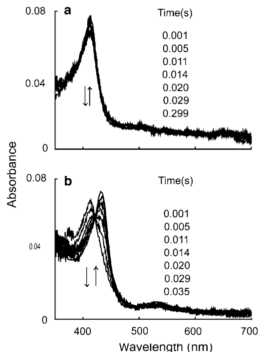
Figure 6 Melatonin facilitates direct conversion of EPO-Fe(III) to Compound II. Absorbance spectra of EPO recorded by diode-array, stopped-flow in the absence (a) and the presence of 100 μM melatonin (b). Experiments were performed under aerobic conditions when phosphate buffer (200 mM, pH 7) containing 1.9 μM EPO and 140 μM Br - in the absence (a) and the presence of 200 μM melatonin (b), was rapidly mixed with a buffer solution supplemented with 40 μM H 2 O 2 at 10 °C. The time of each collected spectrum after initiating the reaction is indicated in each figure in seconds. Arrows indicate the direction of spectral change over time. EPO, eosinophil peroxidase.
