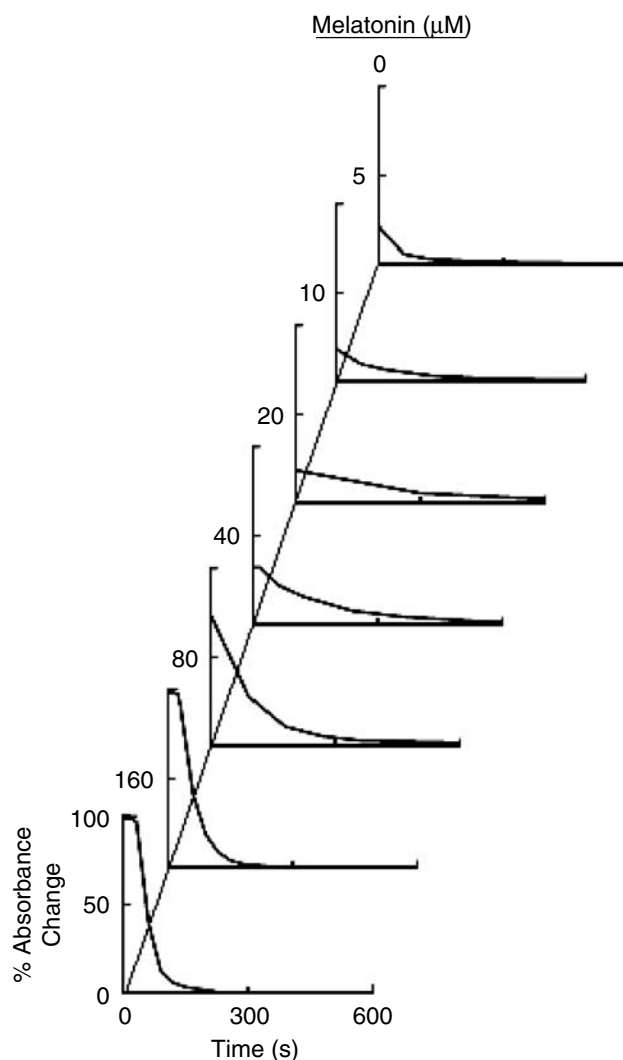
Figure 7 Effect of melatonin concentration on EPO Compound II formation during steady-state catalysis in the presence of plasma levels of Br - . A solution containing sodium phosphate buffer (200 mM, pH 7) supplemented with 2 μM EPO, 200 μM NaBr, and increasing concentrations of melatonin, was rapidly mixed with an equal volume of buffer containing 40 μM of H 2 O 2 EPO-Fe(III) at 10 °C. The time course of EPO Compound II formation during steady-state catalysis was monitored by observing spectral changes at 432 nm. The final concentration of melatonin in the mixture is indicated. Note that even in the presence of physiological levels of the competing substrate Br - , melatonin significantly enhances the overall level of EPO Compound II formed during steady-state catalysis. Data represent the mean of triplicate determinations from an experiment performed three times. EPO, eosinophil peroxidase.
