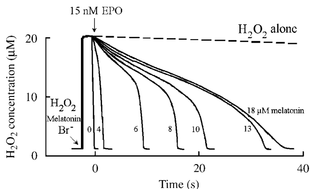
Figure 1 Melatonin inhibits H 2 O 2 consumption by EPO in the presence of Br - . A typical recording by an H 2 O 2 -selective electrode demonstrating auto-reduction of H 2 O 2 (20 µM) following addition to stirred phosphate buffer (200 mM; pH 7) supplemented with 70 µM Br - , at 25 °C (dashed line). Addition of 20 µL (15 nM final concentration) of EPO solution to the H 2 O 2 /Br - stirred buffer caused rapid H 2 O 2 consumption. Addition of 20 µL (15 nM final concentration) EPO solution to the H 2 O 2 /Br - solution supplemented with increasing melatonin concentrations 4, 6, 8, 10, 13 and 18 µM (solid lines from left to right, respectively) causing slower H 2 O 2 removal. Tracings shown are from a typical experiment performed at least three times. EPO, eosinophil peroxidase.
