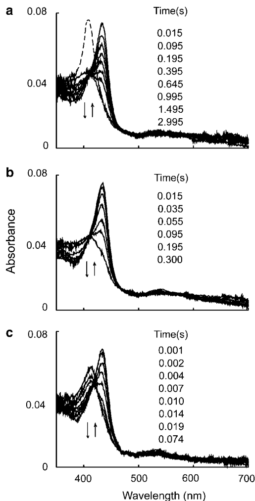
Figure 3 Melatonin accelerates the conversion rates of EPO Compound I to Compound II. Absorbance spectra of EPO recorded by diode array stopped-flow in the absence (a) and in the presence of 10 \mu M (b) and 160 \mu M melatonin (c). Experiments were performed under aerobic conditions when a phosphate buffer solution (200 mM, pH 7) containing 1.6 \mu M EPO in the absence and presence of 20 and 320 \mu M melatonin was rapidly mixed with a buffer solution supplemented with 40 \mu M H_2O_2 at 10 °C as described under Methods. The time of each collected spectrum after initiating the reaction is indicated in each figure in seconds. Arrows indicate the direction of spectral change over time. The dashed line spectrum represents the enzyme as isolated. EPO, eosinophil peroxidase.
