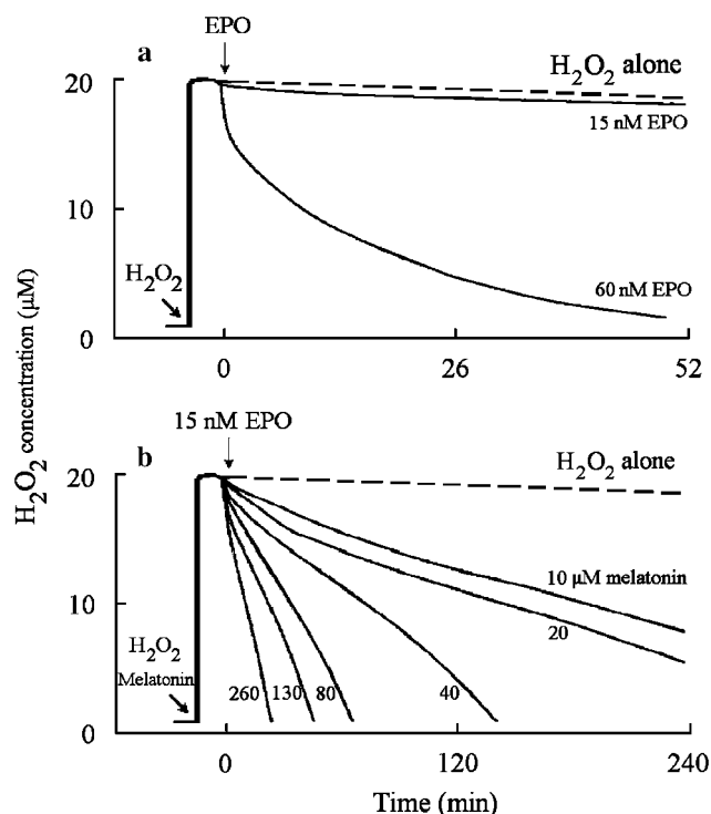
Figure 2 Effect of melatonin on H_2O_2 consumption by EPO in the absence of Br^- . (a) A typical recording by an H_2O_2 -selective electrode demonstrating the auto-reduction of H_2O_2 (20 \mu M ) following addition to stirred phosphate buffer (200 mM; pH 7), at 25 °C (dashed line). Solid lines represent the H_2O_2 consumption as a function of time after the addition of 15 and 60 nM EPO. (b) The effect of increasing melatonin concentration on H_2O_2 consumption rate after the addition of 15 nM EPO to a stirred buffer solution supplemented with 20 \mu M H_2O_2 and the indicated concentration of melatonin on the solid lines. Tracings shown are from a typical experiment performed at least three times. EPO, eosinophil peroxidase.
